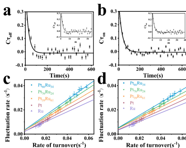
Fig. 4 Autocorrelation function C\tau_{\text{off}}(t) (a) and C\tau_{\text{on}}(t) (b) of the reaction time \tau from turnover trajectories of \text{Pt}_{66}\text{Ru}_{34} nanocatalysts. Inset: autocorrelation function of the \tau_{\text{off}} (a) and \tau_{\text{on}} (b) from the turnover trajectory of a single \text{Pt}_{66}\text{Ru}_{34} nanoparticle; the solid line is a single exponential fit. Autocorrelation function C\tau_{\text{off}}(t) (a) and C\tau_{\text{on}}(t) (b) of the reaction time \tau from turnover trajectories of \text{Pt}_{66}\text{Ru}_{34} nanocatalysts. The x-axis was converted from the turnover index m to real time using the average turnover time of each nanoparticle. The solid line is a single exponential fit. Dependence of the activity fluctuation rates of (c) \tau_{\text{off}} and (d) \tau_{\text{on}} on the reaction rates. All experiments are conducted in a \text{H}_2 -saturated solution of 10 nM resazurin.
