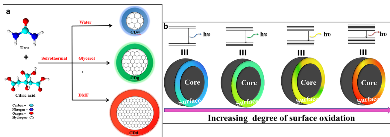
Fig. 2 (a) Full-colour fluorescent CDs depicting size-dependent emission 51 and (b) full-colour luminescent CDs with a surface-state-controlled emission. 57
