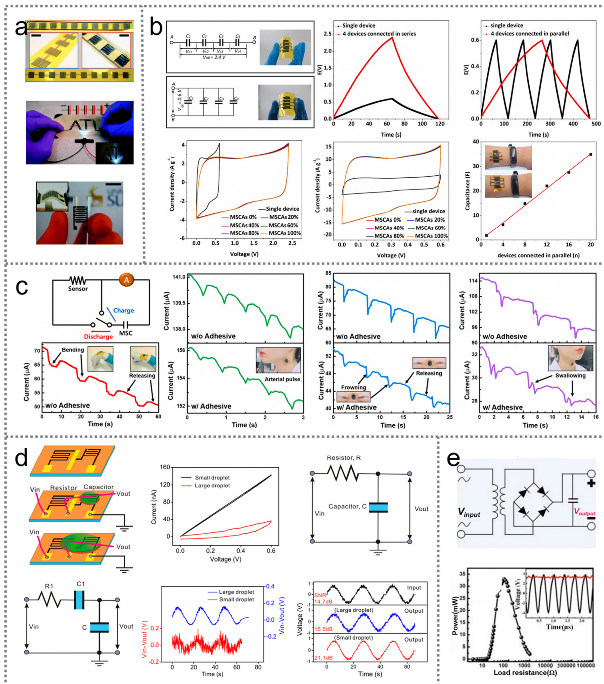
Fig. 9 Applications of PMSCs including energy storage devices, sensors and filters. (a) Digital photographs of 10 IPNiO MSCs connected in parallel and series configurations, then used as the energy storage unit for LEDs. Reproduced with permission. 72 Copyright 2019, Royal Society of Chemistry. (b) Electrochemical performance and flexibility of PMSCs with series and parallel connections. Reproduced with permission. 79 Copyright 2021, Elsevier. (c) Schematic diagram of the integrated system and the strain measurement induced by bio-signals including arterial pulse, frowning and swallowing. Reproduced with permission. 62 Copyright 2021, Elsevier. (d) The fsrGO MSCs applied in RC filter circuits. Reproduced with permission. 101 Copyright 2018, American Chemical Society. (e) Schematic circuit diagram of the wireless charging unit and corresponding output power. Reproduced with permission. 85 Copyright 2020, Elsevier.
