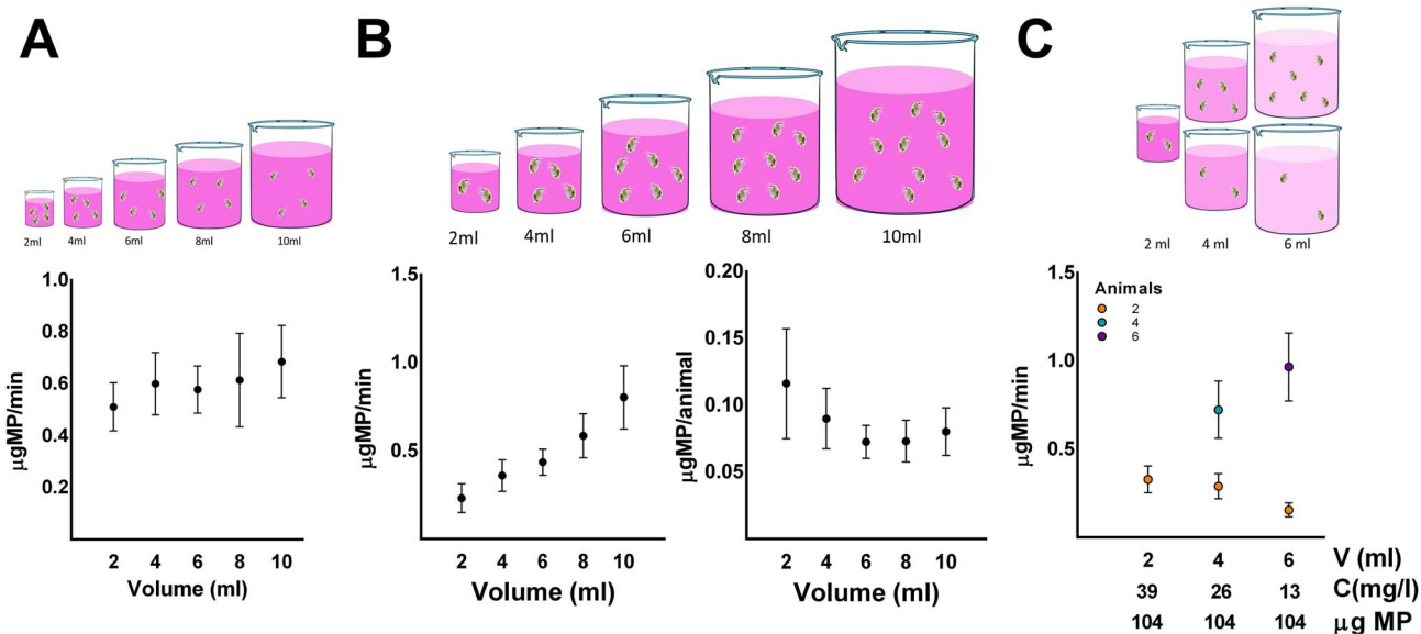
Fig. 2 Optimization of the volume of the feeding assay. (A) Four animals were incubated in different volumes of well plates with the same initial concentration of microparticle (13 mg \text{l}^{-1} ). (B) A different number of animals were used for different volumes (2, 4, 6, 8, and 10 ml) with the same concentration of microparticle (13 mg \text{l}^{-1} ). The results are expressed in \mu\text{g} microparticles per min and \mu\text{g} microparticles per animal (C) The experiment includes two parts of different volume/animal ratios. In the first part same number of animals, and the second part different number of animals were incubated in different volumes and concentrations of microparticles, as shown in the figure. The concentration of microparticle in the supernatant was measured in 10 minute intervals for 60 minutes, and the feeding rate was calculated. Data represent average \pm standard deviation ( N = 4 ).
