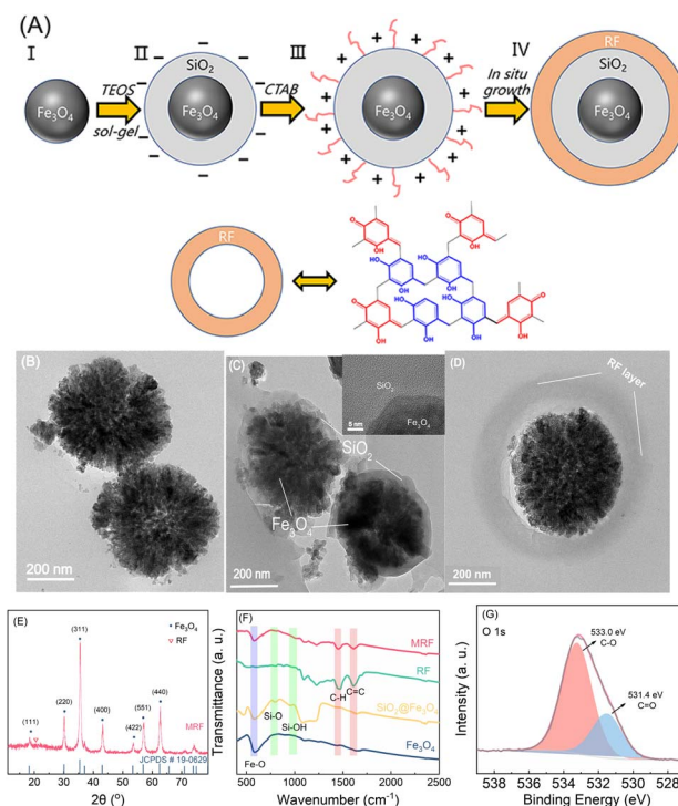
Fig. 1 (A) Schematic synthetic procedure of the magnetic resorcinol-formaldehyde photocatalysts; (B)–(D) TEM images of (B) \text{Fe}_3\text{O}_4 particles, (C) \text{Fe}_3\text{O}_4@ \text{SiO}_2 (inset: HRTEM image at the core-shell interface), and (D) MRF microspheres; (E) XRD patterns of MRF; (F) FTIR spectra of various materials; (G) high-resolution O 1s XPS spectrum of MRF.
