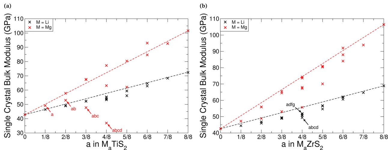
Fig. 11 Variation of the single crystal bulk modulus with intercalant concentration for \text{TiS}_2 (a) and \text{ZrS}_2 (b). Data for both lithium and magnesium intercalation is presented. A straight line (dashed) connecting the bulk modulus of pristine and fully-intercalated structures has been included for visual aid.
