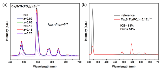
Fig. 6 (a) PL spectra of phosphor \text{Ca}_8\text{SrTb}(\text{PO}_4)_7:xEu^{2+} ( x = 0, 0.02, 0.05, 0.10, 0.15 , and 0.20 ) at 365 nm excitation. (b) IQE and EQE of phosphor \text{Ca}_8\text{SrTb}(\text{PO}_4)_7:0.1Eu^{2+} at 320 nm excitation.
