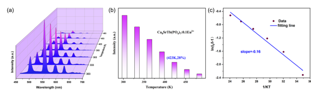
Fig. 7 (a) Temperature-dependent PL spectra ( \lambda_{\text{ex}} = 365 nm) of \text{Ca}_8\text{SrTb}(\text{PO}_4)_7:0.1Eu^{2+} in the 303–483 K temperature range. (b) Emission intensity of \text{Ca}_8\text{SrTb}(\text{PO}_4)_7:0.1Eu^{2+} with increasing temperature. (c) Relationship between \ln(I_0/I - 1) and 1/kT of \text{Ca}_8\text{SrTb}(\text{PO}_4)_7:0.1Eu^{2+} .
