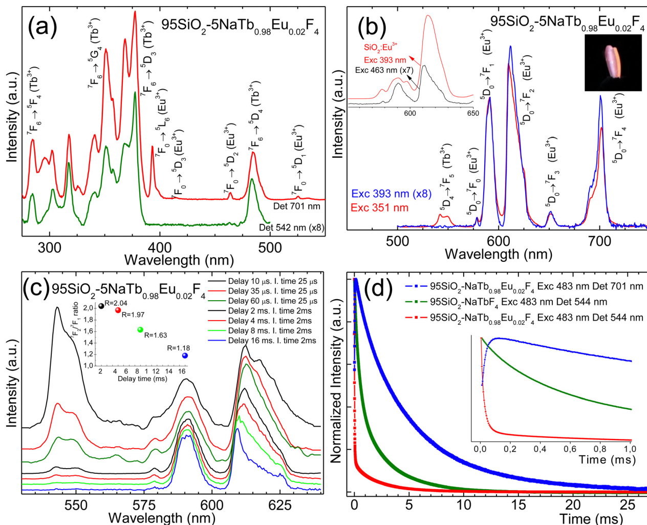
Fig. 5 (a). Excitation spectra of the nGC with composition 95\text{SiO}_2-5\text{NaTb}_{0.98}\text{Eu}_{0.02}\text{F}_4 , detecting at 542 and 701 nm, corresponding to the ^5\text{D}_4 \rightarrow ^7\text{F}_5 and ^5\text{D}_0 \rightarrow ^7\text{F}_4 transitions of \text{Tb}^{3+} and \text{Eu}^{3+} ions, respectively. Spectra have been normalized to the ^7\text{F}_6 \rightarrow ^5\text{D}_4 transition of \text{Tb}^{3+} ions. (b) Emission spectra exciting at 351 and 393 nm, corresponding to the ^7\text{F}_6 \rightarrow ^5\text{G}_4 and ^7\text{F}_0 \rightarrow ^5\text{L}_6 transitions of \text{Tb}^{3+} and \text{Eu}^{3+} , respectively. Spectra have been normalized to the ^5\text{D}_0 \rightarrow ^7\text{F}_1 transition of \text{Eu}^{3+} ions. Right inset shows a digital photograph of the spectra exciting at 351 nm. Left inset shows, emission spectra for nGC exciting \text{Eu}^{3+} ions at 463 nm and for \text{Eu}^{3+} -doped glass, exciting at 393 nm. (c) Delayed emission spectra exciting at 351 nm, with indicated delay and integration times, normalized at ^5\text{D}_0 \rightarrow ^7\text{F}_1 transition of \text{Eu}^{3+} ions. Inset shows long delay asymmetry ratios. (d) Luminescence decay curves of \text{Tb}^{3+} ions in 95\text{SiO}_2-5\text{NaTbF}_4 (exciting at 483 nm and detecting at 544 nm) and 95\text{SiO}_2-5\text{NaTb}_{0.98}\text{Eu}_{0.02}\text{F}_4 nGCs (exciting at 483 nm and detecting at 544 and 701 nm). Inset shows a magnification at short decay times.
