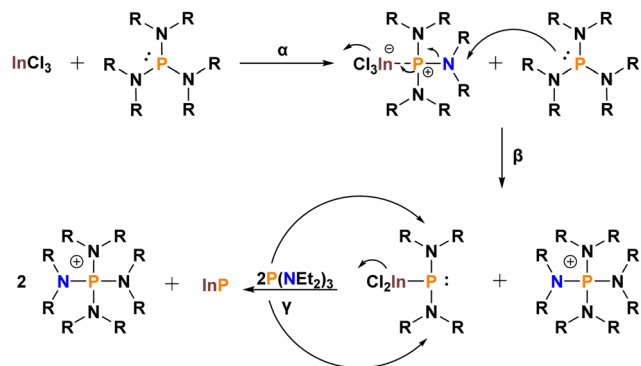
Scheme 2 Proposed mechanism for InP formation from \text{P}[\text{In}(\text{Et})_2]_3 .
