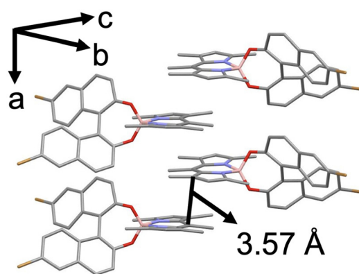
Fig. 3 Single-crystal structures of \pi -stacking between two neighbouring R-0Ph-B-BODIPY units. Black line: \pi -stacking distance: 3.57 Å.
