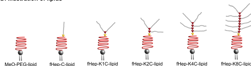
Fig. 1 Overview of fHep-lipid synthesis. (A) Unfractionated heparin is treated with \text{HNO}_2 to fragment the heparin. (B) A linker with different numbers ( n = 0, 1, 2, 4, 8 ) of lysine (K) and one cysteine (C), KnC, is conjugated to a maleimide-1,2-dipalmitoyl- sn -glycero-3-phosphoethanolamine (DPPE)-PEG5k-lipid via the thiol–maleimide Michael addition click reaction. (C) The fragmented heparin is then conjugated to the KnC-lipid via the available amine groups on the KnC-lipids. The amine groups allow for conjugation to an aldehyde group on fragmented heparin via Schiff chemistry, followed by reduction by sodium cyanoborohydride ( \text{NaCNBH}_3 ). (D) Illustration of the lipids used in this study.
