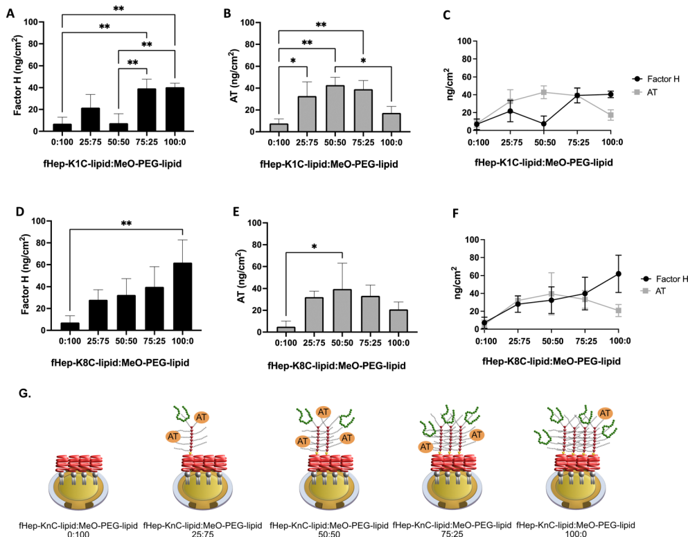
Fig. 3 QCM-D analysis of interaction with purified factor H and AT. Analysis of different ratios of fragmented-heparin-conjugated lipids (fHep-lipids): MeO-PEG-lipids (0:100, 25:75, 50:50, 75:25, and 100:0), followed by flowing of 25 \mu\text{g mL}^{-1} factor H and then 25 \mu\text{g mL}^{-1} antithrombin (AT). (A) Quantification of the amount of factor H bound to different ratios of fHep-K1C-lipid: MeO-PEG-lipid, (B) quantification of the amount of AT bound to different ratios of fHep-K1C-lipid: MeO-PEG-lipid, (C) summary of the amount of factor H and AT bound to different ratios of fHep-K1C-lipid: MeO-PEG-lipid, (D) quantification of the amount of factor H bound to different ratios of fHep-K8C-lipid: MeO-PEG-lipid, (E) quantification of the amount of AT bound to different ratios of fHep-K8C-lipid: MeO-PEG-lipid, and (F) summary of the amount of factor H and AT bound to different ratios of fHep-K8C-lipid: MeO-PEG-lipid. For all experiments, n = 3 . (G) Illustration of factor H (green) and AT binding (orange) to different ratios of fHep-KnC-lipids: MeO-PEG-lipids (0:100, 25:75, 50:50, 75:25, and 100:0).
