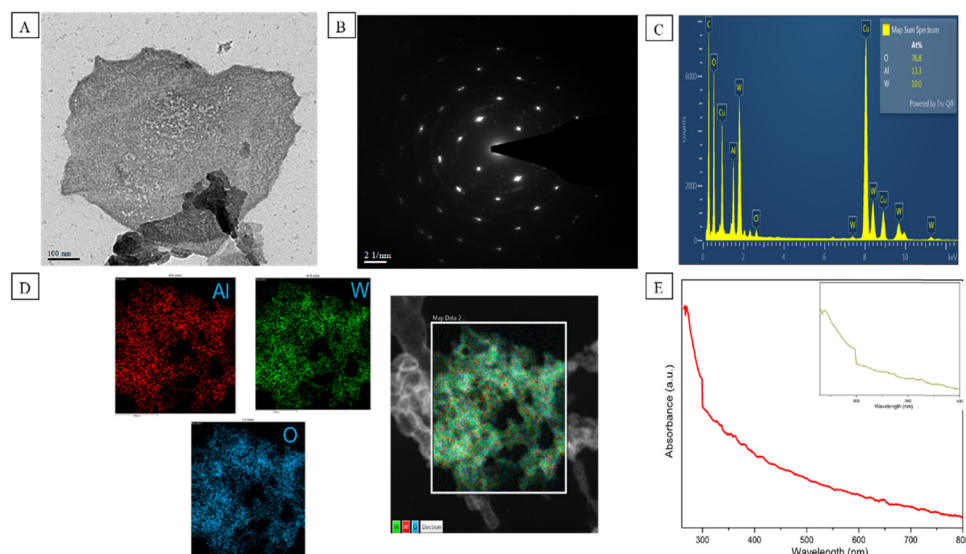
Fig. 2 Characterization of the Al–W nanosheets (A) surface morphology showing layered nanostructure, (B) SAED pattern showing perfect crystalline phases, (C) elemental ratios shown in EDS pattern, (D) high-angle annular dark-field scanning transmission electron microscopy image of Al–W nanosheets, showing the pattern for elements W (green color), Al (red color), O (blue color), and single element mapping of W (green color), O (blue color), and Al (red color), (E) UV spectra of Al–W nanosheets (zoom-in image in the inset shows a hump at 270 nm).
