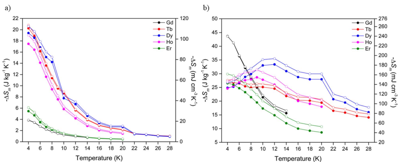
Fig. 3 Magnetic entropy changes of the \text{Ln}(\text{OH})_3 series for (a) \Delta B = 1.0 \text{ T} and (b) \Delta B = 5.0 \text{ T} . The filled and open symbols denote mass and volumetric entropy units respectively.
