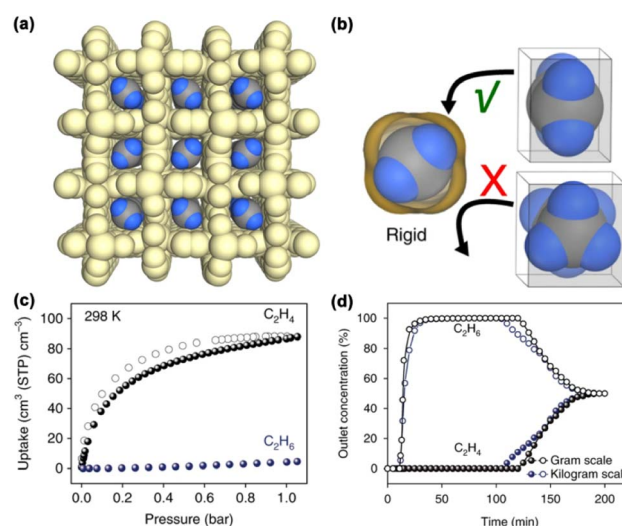
Fig. 9 (a) View of the crystal structure and packing diagram of \text{C}_2\text{H}_4 @UTSA-280. (b) Schematic illustration of size/shape sieving based on the minimum cross-sectional area of \text{C}_2\text{H}_4 and \text{C}_2\text{H}_6 molecules. (c) Single-component adsorption/desorption isotherms of \text{C}_2\text{H}_4 and \text{C}_2\text{H}_6 at 298 K. (d) Comparison of experimental breakthrough curves for a 50/50 \text{C}_2\text{H}_4/\text{C}_2\text{H}_6 mixture on UTSA-280 synthesized on different scales. Reproduced from ref. 59 with permission from copyright 2018, Springer Nature.
