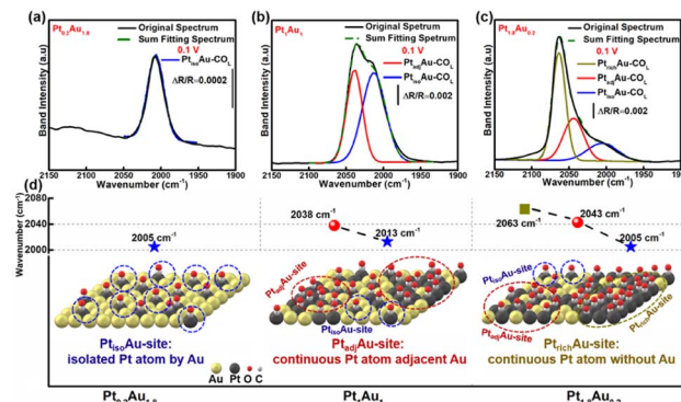
Fig. 3 (a)–(c) Peak fitting of the \text{CO}_L bands of the PtAu model films at 0.1 V: (a) \text{Pt}_{0.2}\text{Au}_{1.8} , (b) \text{Pt}_1\text{Au}_1 and (c) \text{Pt}_{1.8}\text{Au}_{0.2} . (d) Wavenumbers of the fitting peak positions and \text{CO}_{\text{ad}} diagrams of the surface fine structures of the PtAu model films: \text{Pt}_{0.2}\text{Au}_{1.8} left figure, \text{Pt}_1\text{Au}_1 middle figure, \text{Pt}_{1.8}\text{Au}_{0.2} right figure.
