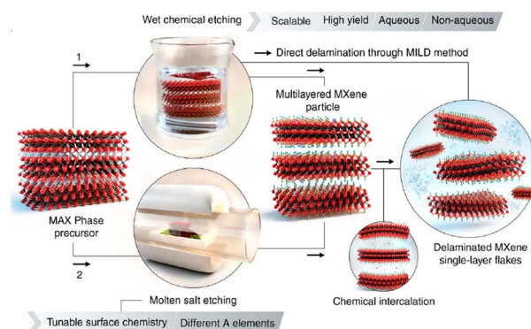
Fig. 4 Schematic representation of two etching strategies to remove the A layers from MAX phases to produce multi-layered MXenes and delaminated single layer flakes. Reproduced with permission from ref. 67, Copyright 2021 Science.
