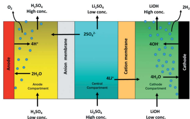
Fig. 16 American Manganese RecycLiCo™ process, a three compartment membrane electrodialysis cell for generating LiOH and H 2 SO 4 (reproduced from ref. 67 with permission from Taylor and friends, copyright 2021).
