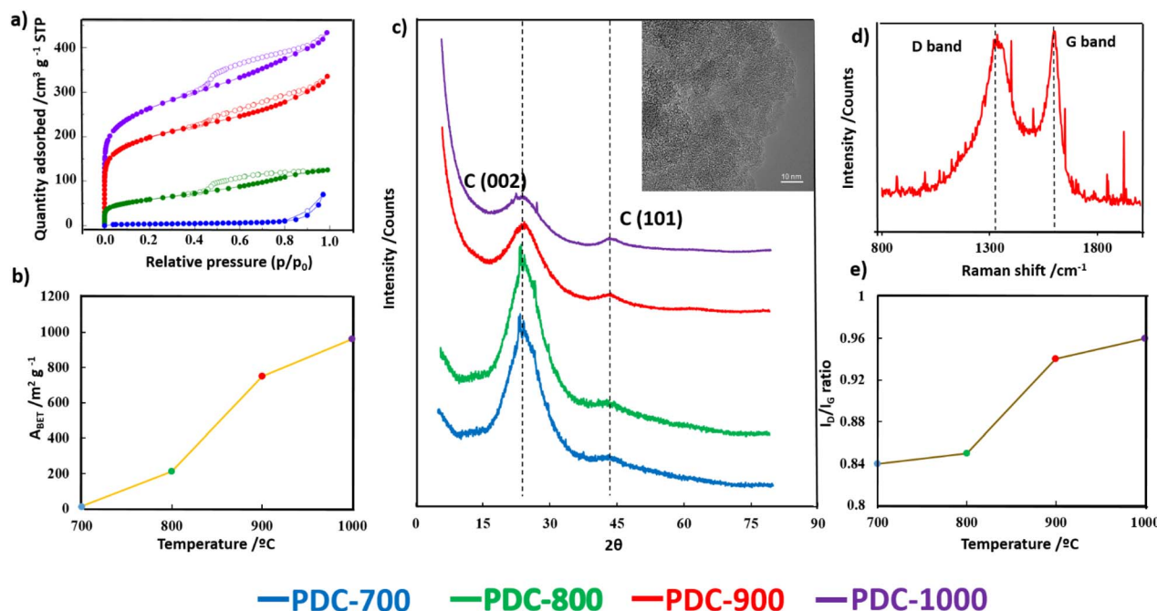
Fig. 2 (a) N 2 adsorption (full symbols) – desorption (empty symbols) isotherms of the PDC- T series; (b) plot of A BET obtained from N 2 adsorption isotherms; (c) XRD patterns of the PDC- T series and TEM image of PDC-900 (inset); (d) Raman spectra of PDC-900; and (e) plot of I D / I G ratio obtained from Raman spectra.
