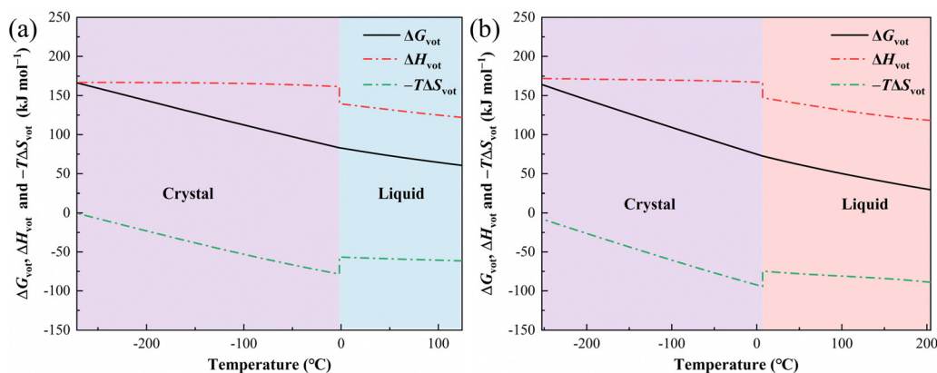
Fig. 7 The enthalpy of vaporization or sublimation ( \Delta H_{vot} ), the -T(K) \times entropy of vaporization or sublimation ( -T\Delta S_{vot} ) and Gibbs free energy of vaporization or sublimation ( \Delta G_{vot} ) of [C_2mim][NTf_2] from -271.71 to 124.35 °C (a) and [C_4mim][NTf_2] from -252.85 to 204.45 °C (b), respectively.
