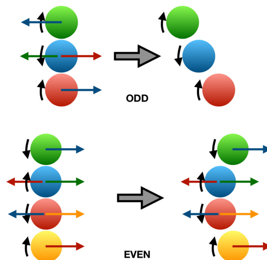
Fig. 11 Schematic diagram explaining the formation of tilted (odd) and bow (even) shaped chains when neighboring particles are perturbed to have angular velocities in opposite directions in the Quincke regime. The black arrows denote the directions of rotation. The colored arrows show the translational velocities induced by rotlet flows generated by the particles of the corresponding colors.
