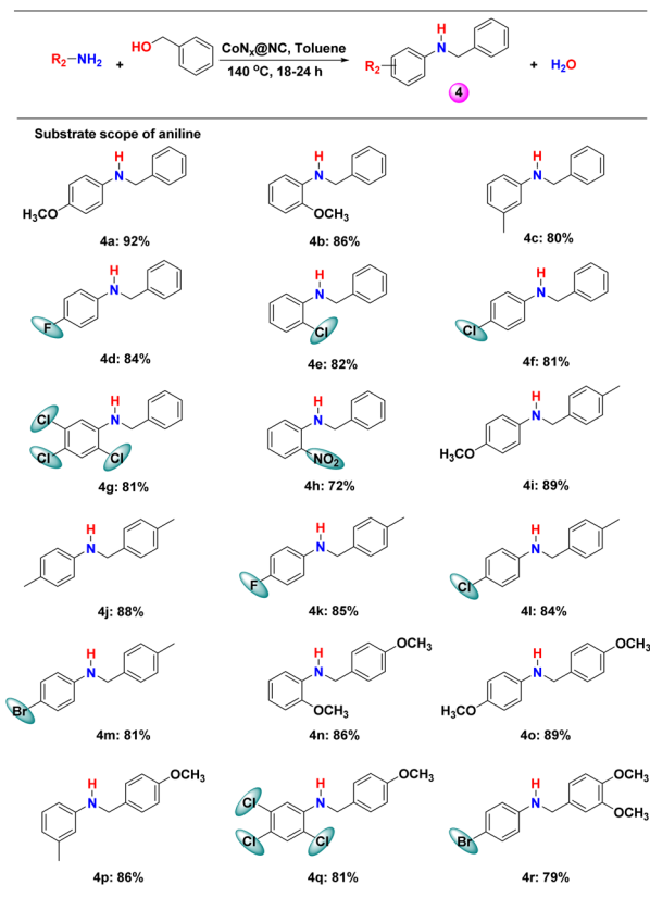
Scheme 3 \text{CoN}_x\text{@NC} catalysed N -alkylation reaction of different anilines with benzyl alcohols. Reaction conditions: 1 mmol substituted benzyl alcohol, 0.5 mmol aniline, 10 mg catalyst, 0.5 mmol tert -BuOK, 2 mL toluene, 140 °C, 24 h. For 4d (18 h), 4e (20 h) and 4f (20 h) optimized at different times.
