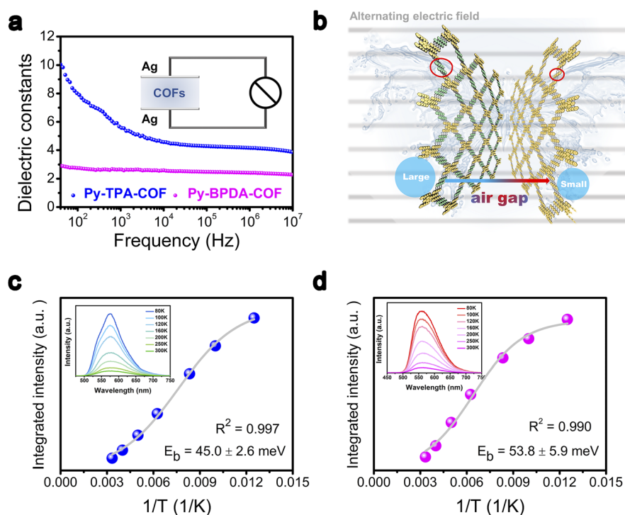
Fig. 2 (a) Dielectric properties of Py-TPA-COF and Py-BPDA-COF dependent on frequency (inset shows a sketch of the flat plate method for measuring the dielectric constant). (b) Diagram of the “air gap” modulation of Py-TPA-COF and Py-BPDA-COF in an alternating electric field. (c) and (d) Temperature inverse versus Arrhenius equation for the integrated photoluminescence (PL) emission intensity of (c) Py-TPA-COF and (d) Py-BPDA-COF (illustration presents the PL spectrum versus temperature).
