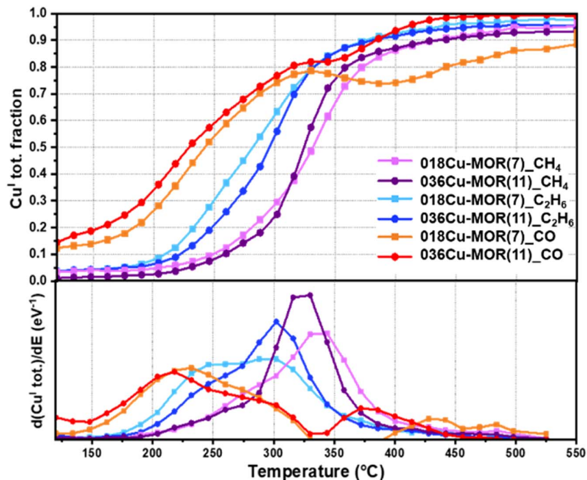
Fig. 3 Comparison of MCR-derived total \text{Cu}^{\text{I}} fraction as a function of temperature for each sample/reactant combination (top panel) in the \text{CH}_4 -, \text{C}_2\text{H}_6 -, and \text{CO} -TPR steps, and corresponding first derivative (bottom panel) to better identify inflection points in the \text{Cu}^{\text{I}} total fraction profile.
