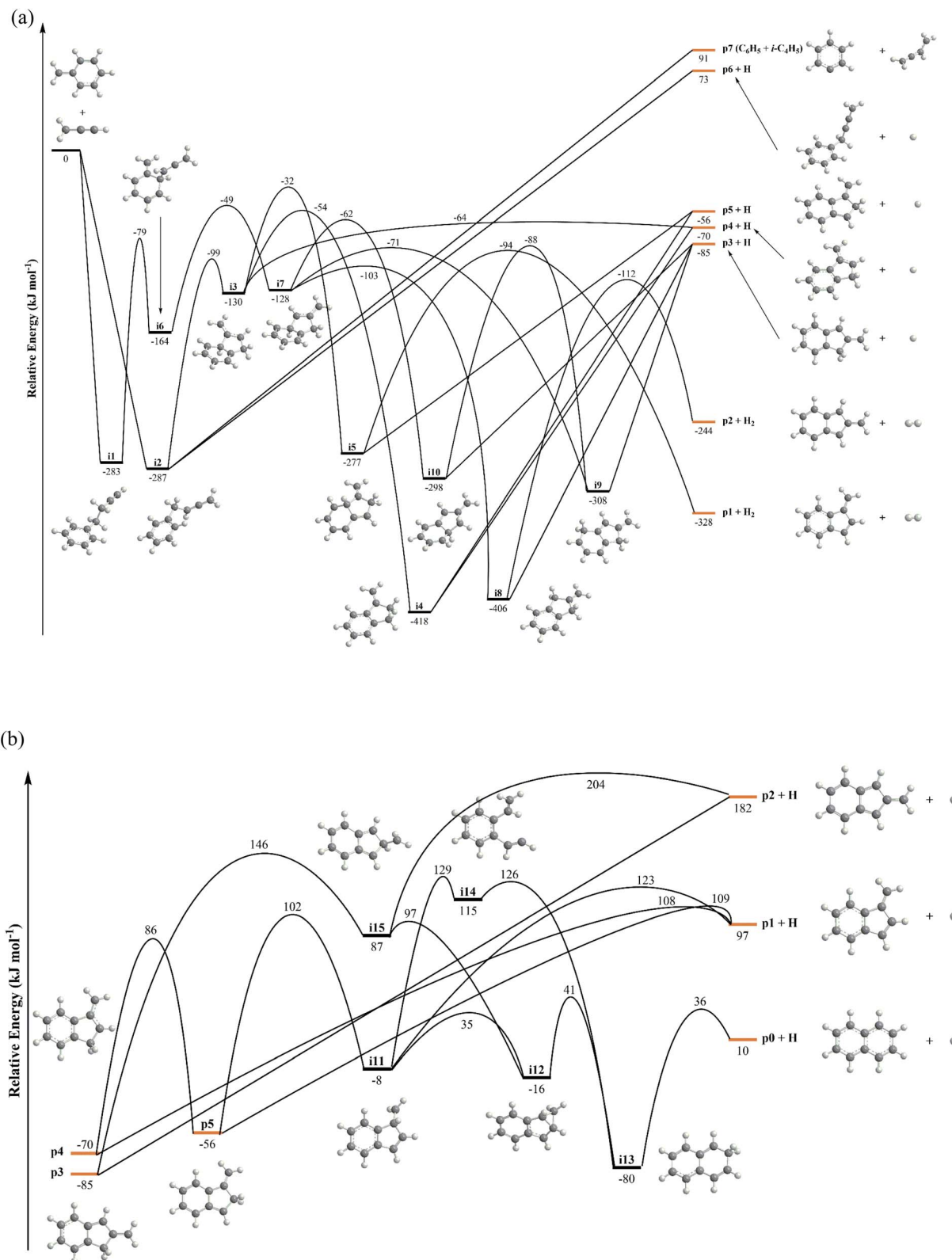
Fig. 4 (a) Main reaction pathways for the benzyl (C 7 H 7 ) plus propargyl (C 3 H 3 ) reaction. All energies are given in kJ mol -1 with respect to the energy of the separated reactants. (b) Main reaction pathways for unimolecular decomposition methylene-indanyl radicals C 10 H 9 (p3–p5). All energies are given in kJ mol -1 with respect to the energy of the initial reactants of the benzyl–propargyl radical–radical reaction. Atoms are colored in black (carbon) and gray (hydrogen).
