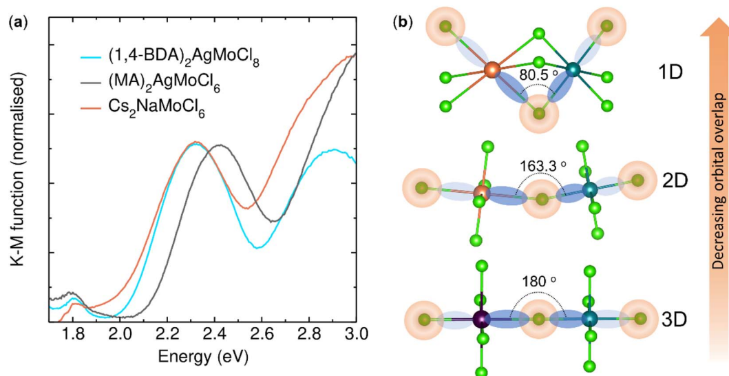
Fig. 5 (a) Optical absorption spectra. (b) Schematic illustration of reduced orbital overlapping between [M^{\text{IV}}\text{Cl}_6]^{5-} and [\text{Mo}^{\text{III}}\text{Cl}_6]^{3-} octahedra due to lattice distortion.
