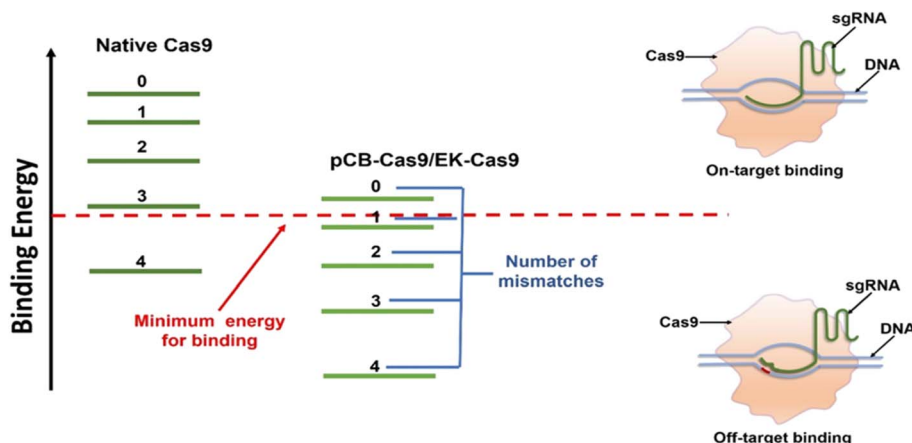
Fig. 2 Mechanism of pCB conjugation or (EK) n peptide fusion in reducing the off-target efficiency of the CRISPR/Cas9 system. The Cas9/sgrRNA complex possesses more energy than what is needed for optimal recognition of its target DNA site, leading to the cleavage of mismatched off-target sites. pCB polymer conjugation (EK) n peptide fusion eliminates the non-specific binding between Cas9/sgrRNA complex and double-strand DNA, thereby decreasing the binding energy. The remained energy is strong enough for on-target binding, but not enough for mismatched binding.
