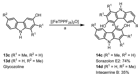
Scheme 3 (FeTPPF 28 ) 2 O-catalyzed synthesis of 4,4'-bicarbazoles. Reaction conditions: a) 13 (0.15 mmol), (FeTPPF 28 ) 2 O ( 5c ) (1.5 mol%), BF 3 ·OEt 2 (20 mol%), CH 2 Cl 2 (15 mL), air, rt.
