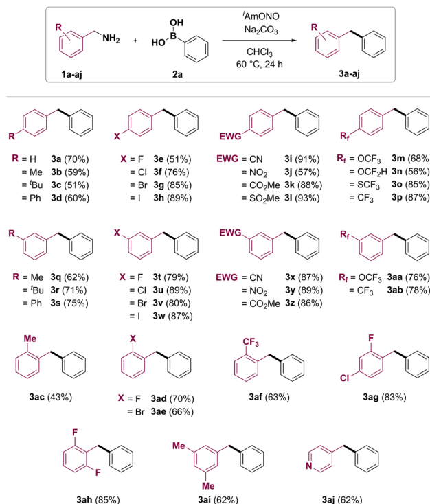
Fig. 2 Benzylamine scope of the deaminative coupling between benzylamines and arylboronic acids. Reaction conditions: benzylamine (1a-aj, 2.0 mmol), phenylboronic acid (2a, 0.5 mmol), isoamyl nitrite (2.5 mmol), sodium carbonate (0.5 mmol), chloroform (1.25 mL), 60 °C, 24 h. Isolated yields after flash column chromatography.
