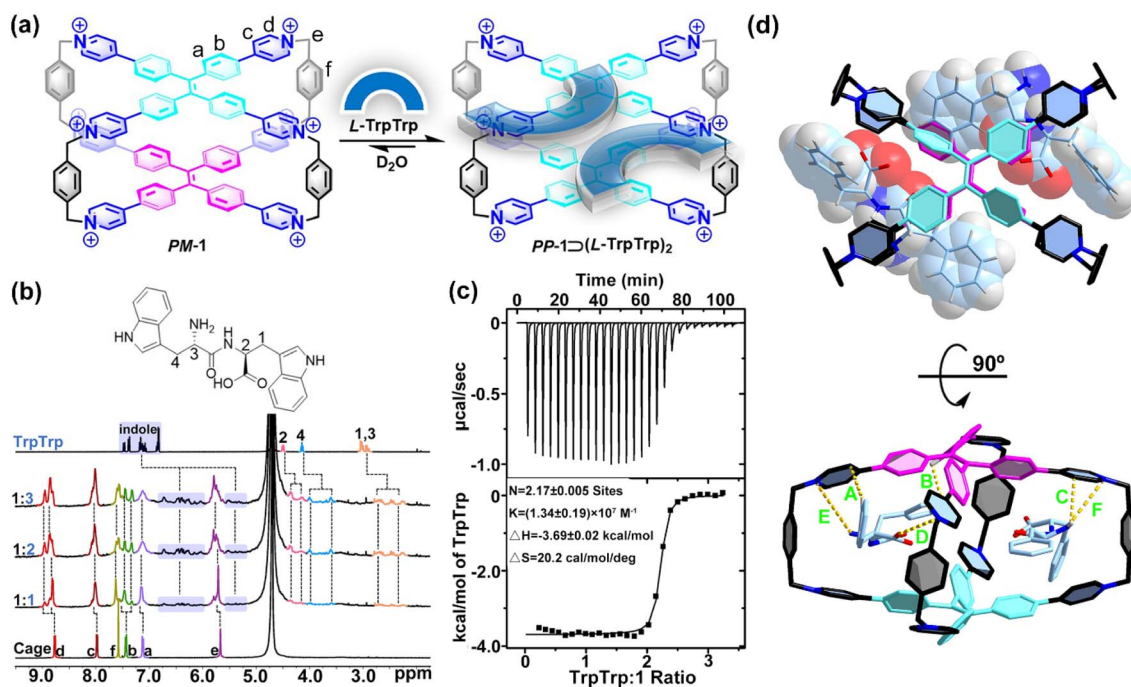
Fig. 2 (a) Schematic representation of the host–guest complexation of PP-1 with L-TrpTrp . (b) ^1H NMR spectra (400 MHz, 298 K, D_2O ) recorded for 1 (0.40 mM) with 1.0–3.0 equiv. of L-TrpTrp . (c) ITC of 1 with L-TrpTrp at 298 K in phosphate buffer (10 mM sodium phosphate, pH = 7.4). (d) Top and side views of the X-ray structure of PM-1 with L-TrpTrp . The dashed lines are key CH\cdots\pi interactions with distances of 2.70 Å (A), 2.35 Å (B) and 2.83 Å (C), electrostatic interactions with distances of 4.44 Å (D), and ion–dipole interactions with distances of 3.85 Å (E) and 4.97 Å (F). Br^- counter ions and hydrogen atoms are omitted for clarity. CCDC number: 2155590† for PM-1 with L-TrpTrp .
