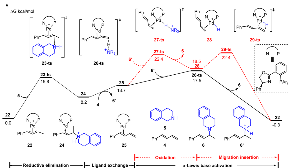
Fig. 6 Reaction energy profile of the cationic Pd(II)-π-allyl mediated Pd-catalyzed hydroamination of aliphatic amine with 1,3-diene.
