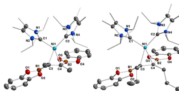
Fig. 4 Molecular structures of [Ni(iPr_2Im^{Me})_2(\eta^2-cis-(Bcat)(Me)C=C(Me)(Bcat))] 15a (left) and [Ni(iPr_2Im^{Me})_2(\eta^2-cis-(Bcat)(H_7C_3)C=C(C_3H_7)(Bcat))] 15b (right) in the solid state (ellipsoids shown at 50% probability level). Hydrogen atoms have been omitted for clarity. For selected bond lengths and angles see ESI Fig. S15 and S16.†
