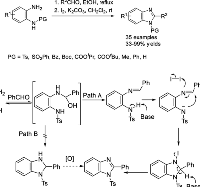
Scheme 74
