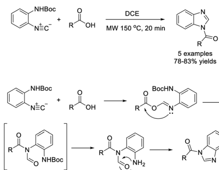
Scheme 143
