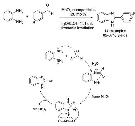
Scheme 7
