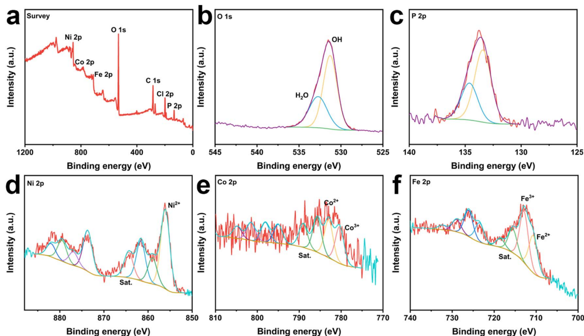
Fig. 2 The survey spectra (a), high-resolution X-ray photoelectron spectra of (b) O 1s, (c) P 2p, (d) Ni 2p, (e) Co 2p, and (f) Fe 2p of CoNiP@NiFe-LDH/NF.
