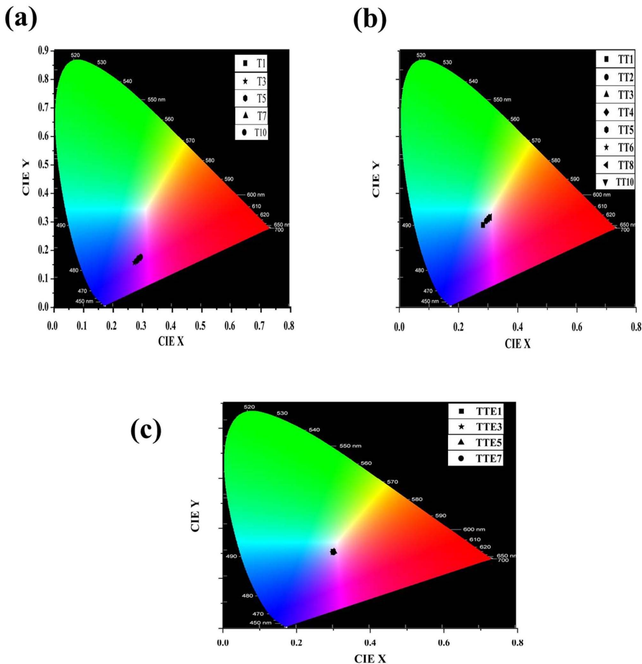
Fig. 14 CIE coordinates of (a) SNB: x\text{Tm}^{3+} , (b) SNB:3 \text{Tm}^{3+} / y\text{Tb}^{3+} and (c) SNB:3 \text{Tm}^{3+} /6 \text{Tb}^{3+} / z\text{Eu}^{3+} samples.
