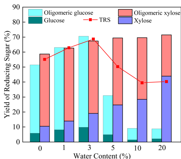
Fig. 3 Effect of water content on TRS yield obtained by hydrolysis of corncob with \text{Sl-C-S-H}_2\text{O}_2 (reaction conditions: 130 °C for 8 h, 0.05 g corncob, 0.05 g catalyst, 2 g [\text{BMIM}][\text{Cl}] ).
