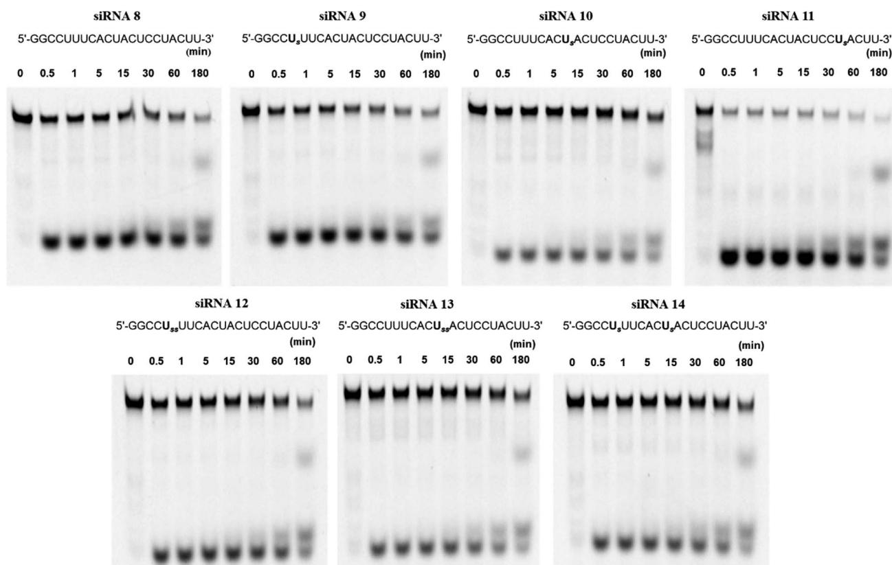
Fig. 3 Degradation profile of siRNAs treated with 5% bovine serum on 15% polyacrylamide gel upon electrophoresis. Fluorescein labeled complementary RNA 13; 3'-UCCGGAAGUGAUGAGGAUG-F-5' was annealed with modified RNAs shown above, to obtain corresponding siRNAs as mentioned. U denotes 4'-PLev-U analog, s denotes spermine and F denotes fluorescein.
