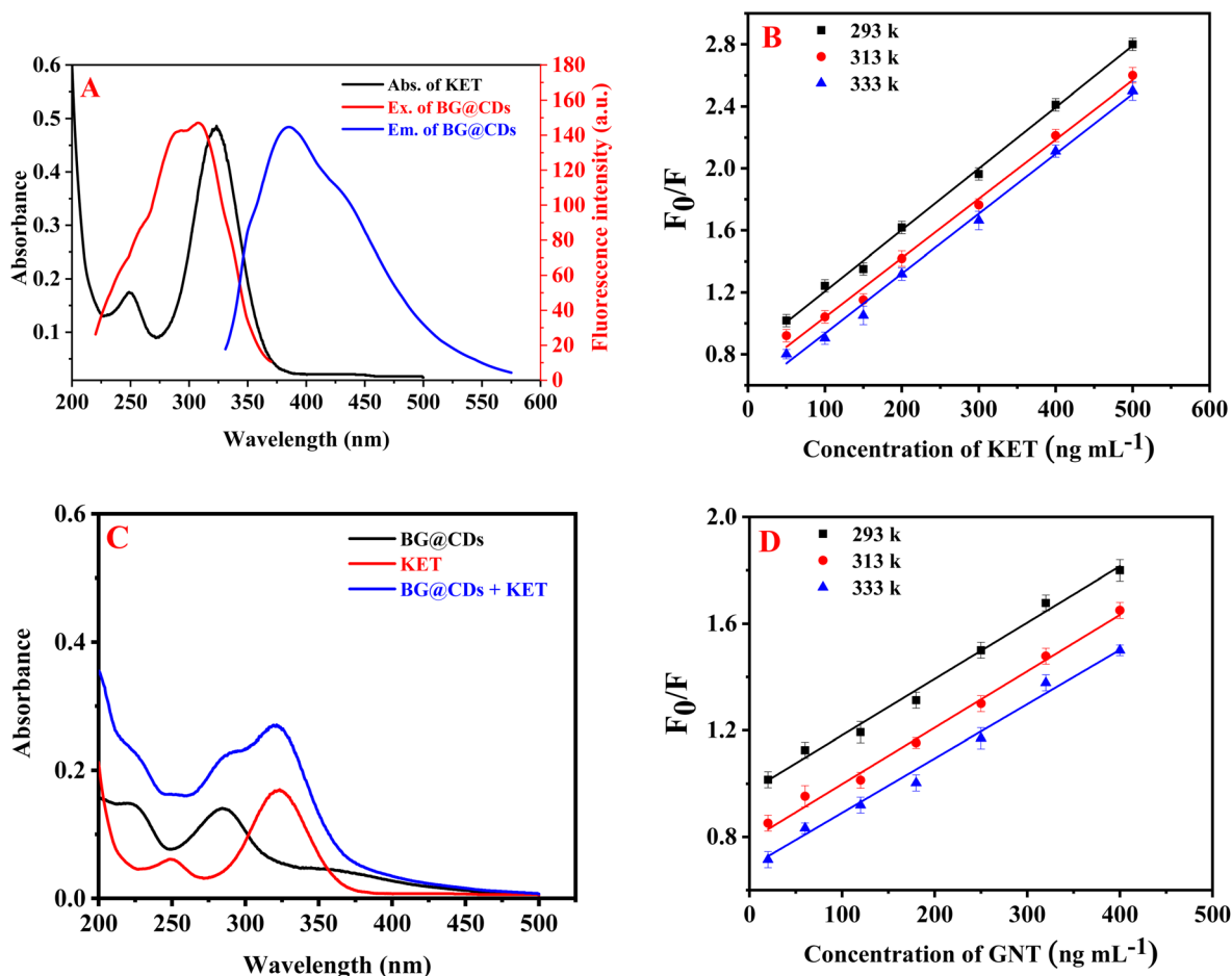
Fig. 4 (A) UV-vis absorption of KET ( 10.0 \mu\text{g mL}^{-1} ) and excitation/emission spectra of the BG@CDs ( 0.1 \text{ mg mL}^{-1} ), (B) Stern–Volmer plots of BG@CDs ( 0.1 \text{ mg mL}^{-1} ) with KET under different temperatures, (C) UV-vis absorption spectra of BG@CDs ( 0.1 \text{ mg mL}^{-1} ), KET ( 5.0 \mu\text{g mL}^{-1} ) and their mixtures, (D) Stern–Volmer plots of EY ( 0.1 \mu\text{g mL}^{-1} ) with GNT under different temperatures.
