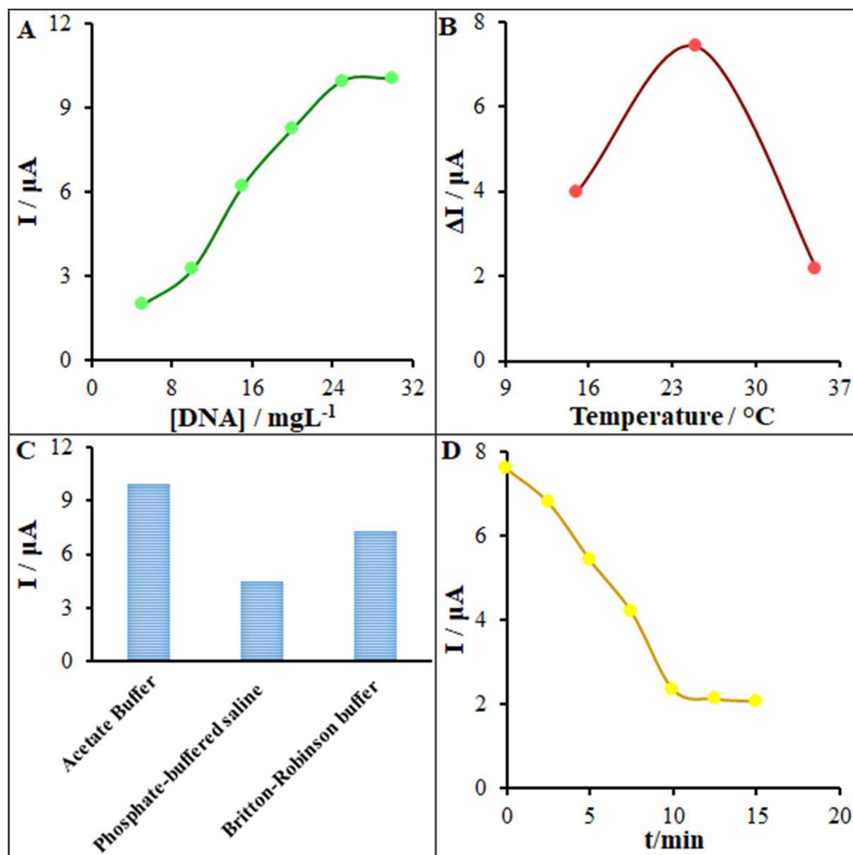
Fig. 9 (A) Oxidation signal plot of guanine vs. ds-DNA concentration (5.0–30.0 \text{mg L}^{-1} ). (B) Plot of guanine oxidation current vs. intercalation solution temperature. (C) Diagram of guanine oxidation current vs. type of buffer solution. (D) Influence of the incubation time of 40.0 \mu\text{M} pemetrexed in ABS (0.5 M, pH 4.8) on the response of ds-DNA/PP/FL-NP Tb 3+ /ZnO/PGE.
