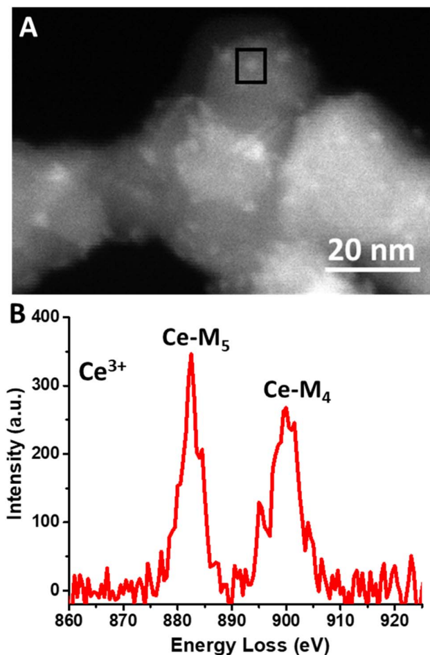
Fig. 5 (A) The square region of the HAADF-STEM image (representing a Ce-carbonate cluster deposited onto \text{TiO}_2 ) was used to acquire the electron energy loss spectrum (EELS) in (B). (B) Cerium EELS of the highlighted Ce(III) carbonate cluster square region deposited onto \text{TiO}_2 in (A).
