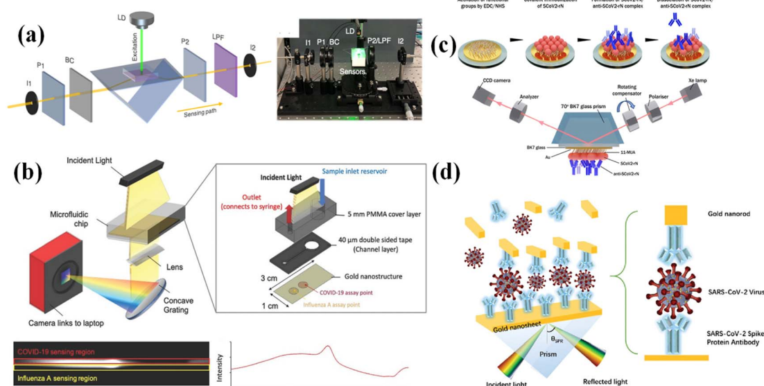
Fig. 6 (a) Schematic and experimental setup of the dual-functional PPT-enhanced LSPR biosensing system. Reproduced with permission from ref. 127. (b) Scheme of the SPR spectral imaging platform integrated with a microfluidic chip. A typical spectral image is shown, and it was obtained from the CCD. Reproduced with permission from ref. 128. (c) Schematic representation of the gold-coated sensor disk (Au-disk) surface modified with antigen SCoV2-rN, which was applied as an interactive surface. Reproduced with permission from ref. 129. (d) The SPR biosensor was designed using a sandwich structure. Reproduced with permission from ref. 130.
