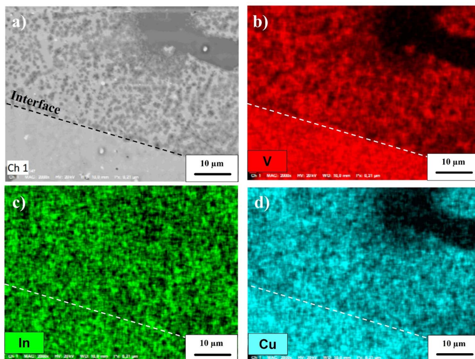
Fig. 8 (a) SEM image of Cu 2 V 2 O 7 thin film after the photocorrosion test (the interface delimits the submerged surface at the top of the image); (b)–(d) colorized elementary maps for vanadium, indium and copper elements, respectively.
