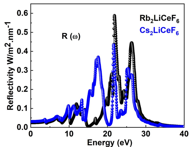
Fig. 7 R(\omega) of M_2LiCeF_6 ( M = Rb and Cs ) compounds.
