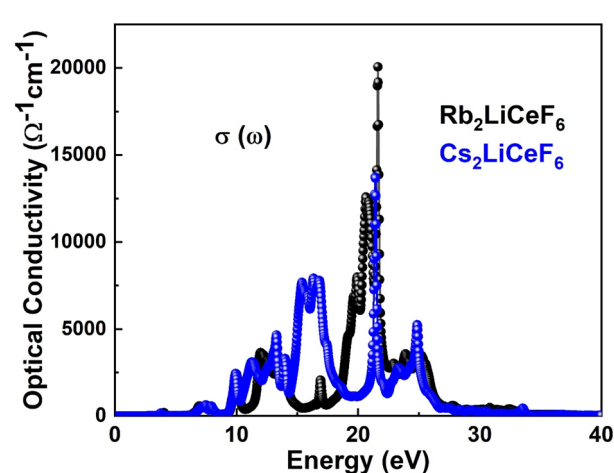
Fig. 8 \sigma(\omega) of M_2LiCeF_6 ( M = Rb and Cs ) compounds.
