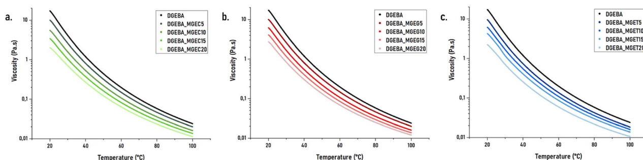
Fig. 3 Viscosity as a function of temperature of DGEBA_MGEC (a), DGEBA_MGE (b) and DGEBA_MGET (c) mixtures.
