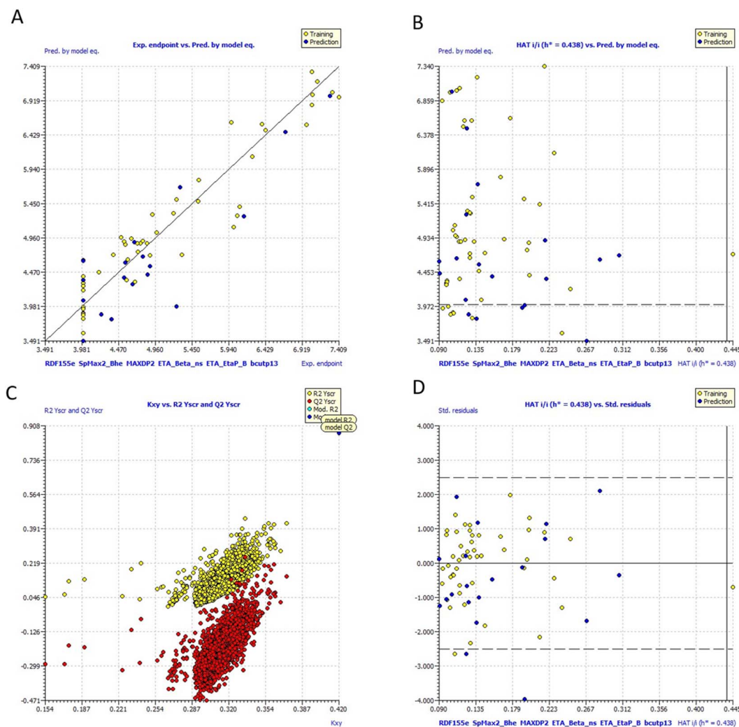
Fig. 10 (a) Graph of experimental vs. Predicted \text{pIC}_{50} values for model 1 (b) Insubria plot for model 1; (c) Y-scrambling plot for model 1 (d) William's plot for model 1.
