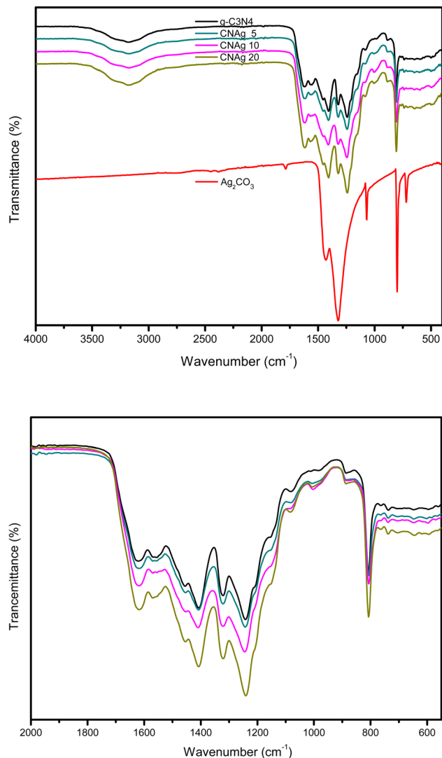
Fig. 3 FTIR spectra of g-C 3 N 4 , Ag 2 CO 3 , CNAg5, CNAg10 and CNAg20 nanocomposites.
