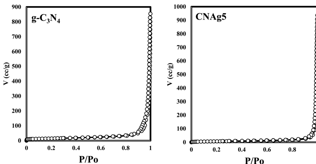
Fig. 4 N 2 -adsorption-desorption isotherms of g-C 3 N 4 and CNAg5.
