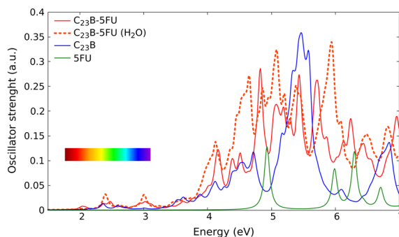
(c) Gas-phase absorption spectra of \text{C}_{23}\text{B} -5FU (red line), \text{C}_{23}\text{B} (blue line) and 5FU (green line). The spectrum of \text{C}_{23}\text{B} -5FU in aqueous solution is reported in dotted red line.
