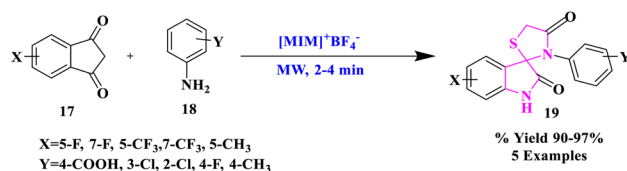
Scheme 4 Synthesis of fluorinated spiro[indole-thiazolidines].
