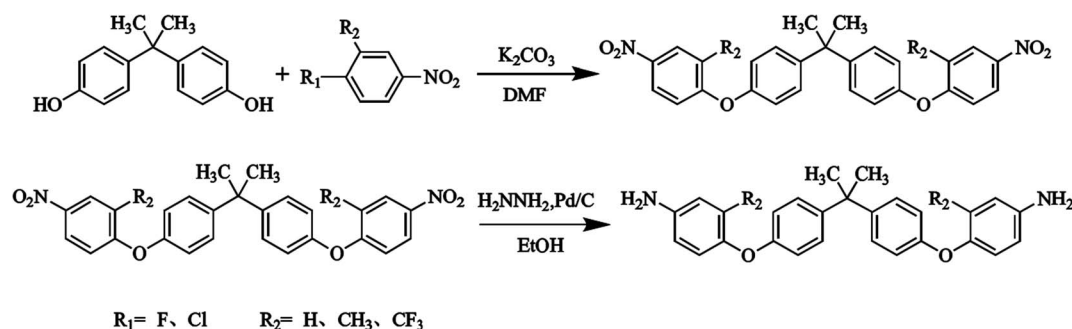
Scheme 1 Synthesis routes of the bisphenol A-containing diamines.
