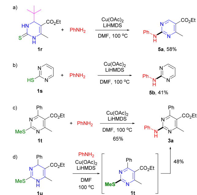
Scheme 4 Control experiments.
