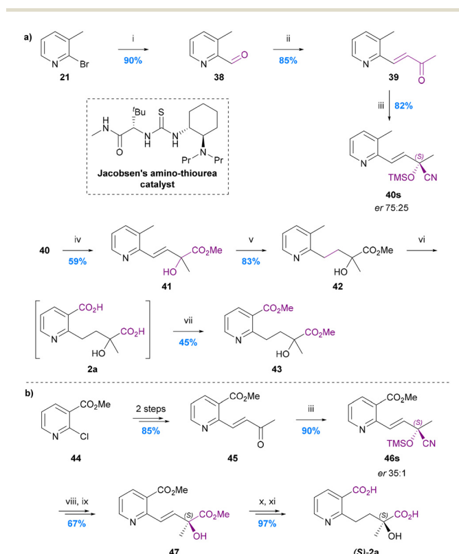
Chart 9 The synthesis of hydroxy wilfordic acid 2a . (a) Seo et al. 2009. 64 (i) t BuLi, DMF, THF, (ii) MeCOCH 2 P(O)(OMe) 2 , NaH, THF, (iii) Jacobsen's amino-thiourea catalyst, TMSCHN 2 , CF 3 CH 2 OH, CH 2 Cl 2 , –78 °C, (iv) 6 M HCl, MeOH, reflux, (v) H 2 , Pd/C, MeOH, (vi) KMnO 4 , H 2 O, reflux, (vii) HCl, MeOH; (b) Seo et al. 2019. 20 (viii) c. HCl, MeOH, 60 °C, (ix) TMSCHN 2 , MeOH, (x) H 2 , Pd/C, MeOH, (xi) LiOH·H 2 O, MeOH/H 2 O.
